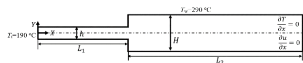
Fig. 1 Geometry of the symmetric planar channel with 1:3 abrupt expansion
