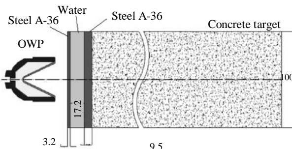
Fig. 2 The test setup according to API-RP43 (dimension mm) [6]
