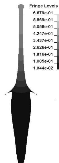
Fig. 8 velocity gradient in jet at 18 \mu s (cm/ \mu s)
