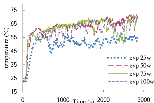
Fig. 4 Evaporator temperature vs. time for heat input
