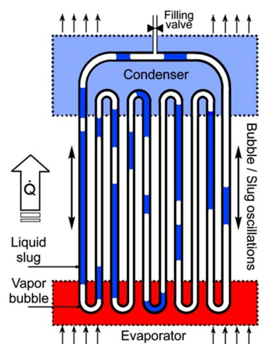
Fig. 1 Schematic of pulsating heat pipe
