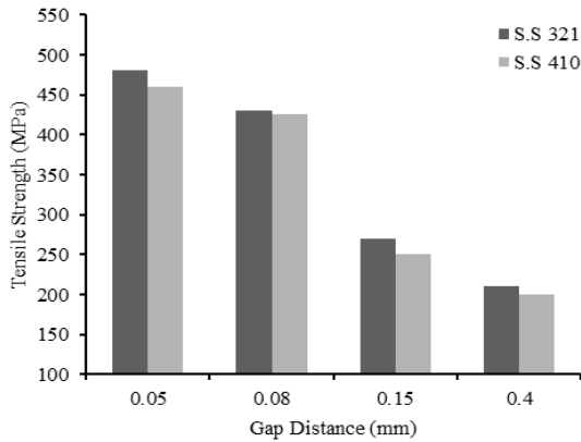
Fig. 9 Tensile strength versus gap distance
