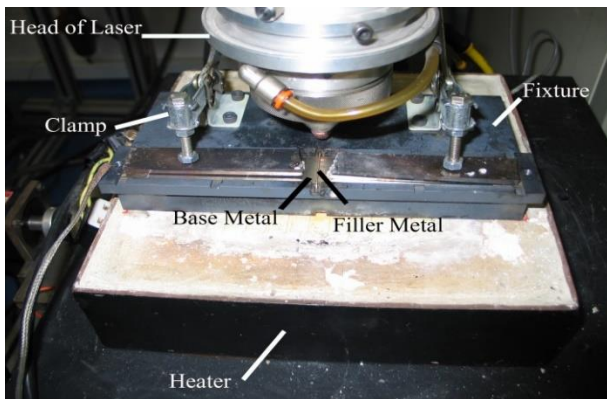
Fig. 1 Experimental setup of laser brazing
