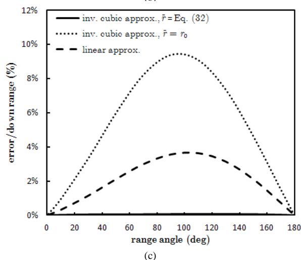
Fig. 4 Error percentage of inverse cubic and linear gravity approximates vs. range angle for stationary targets, a) n = 0 , b) n = 5 , and c) n = 10
