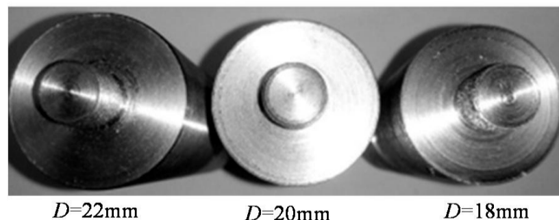
Fig. 2 The tools used by geometry of the threaded pin (Tool shoulder diameter)
