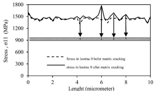
Fig. 15 The graph for changing behavior of the Stress for a [0/90/0] composite with 0.2 mm thickness-along the border of the composite layers and under the effects of the crack
