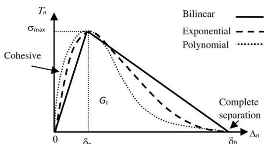
Fig. 2 Three common categories for traction-separation law [26]
