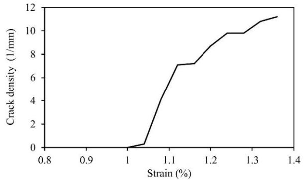
Fig. 13 Crack density graph for a [0/90/0] composite with 0.2 mm thickness under the effects of tensile loading
