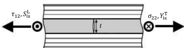
Fig. 16 Crack geometry in a thick embedded 90 degree ply
