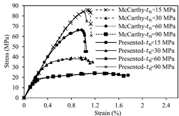
Fig. 7 Fracture behavior of the unit cell under the effect of tensile loading obtained from McCarthy and the presented model in this study with respect to various levels of the stress [31]
