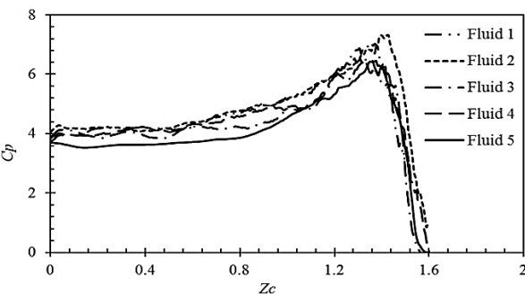
Fig. 17 The distribution of pressure coefficient versus Z_c
