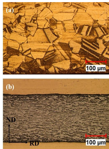
Fig. 5 Microstructure of composite (a) brass and (b) IF steel annealed at 600°C
