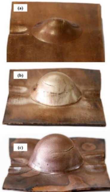
Fig. 11 Stereomicroscopy picture of the Erichsen cup surface of composite in three modes (a) before annealing, annealed at (b) 500°C and (c) 700°C
