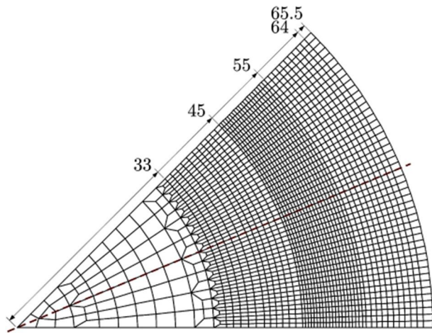
Fig. 3 Partial model 45 degrees
