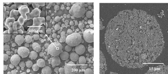
Fig. 2 SEM image of the agglomerated ZrO_2 particles
