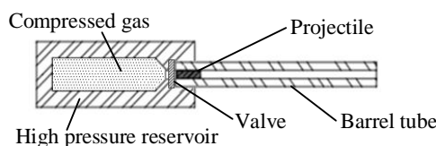
Fig. 1 Scheme of one-stage gas launcher
