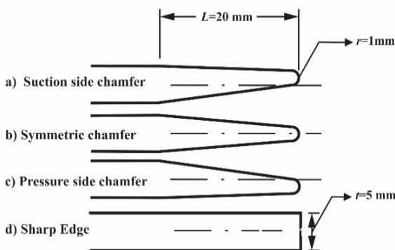
Fig. 8 Details of blade inlet rounding and chamfer
