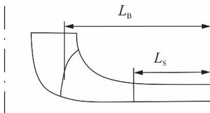
Fig. 7 Impeller meridional view, L_S : splitter blade, L_B : Blade length
