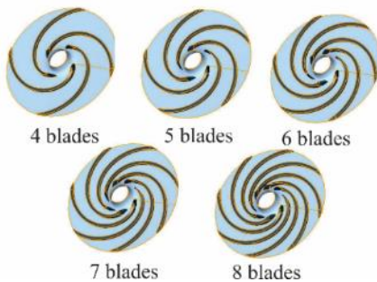
Fig. 6 Blade number.
