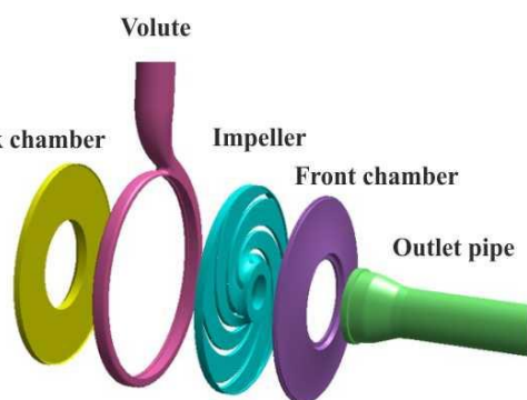
Fig. 2 3D models of flow domain including: outlet pipe, front chamber, impeller, volute, back chamber
