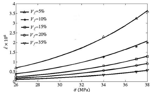
Fig. 10 Creep rate vs. the applied macro stress in axial loading for various VVF
