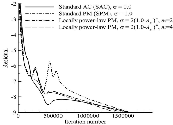
Fig. 15 Effect of the locally power-law PM on convergence rate around the NACA0012 hydrofoil at Re = 1100 , \alpha = 20^\circ
