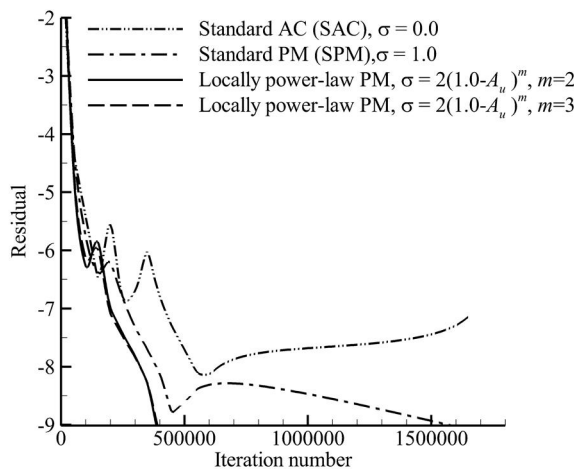
Fig. 18 Effect of the locally power-law PM on convergence rate around the NACA0012 hydrofoil at Re = 1100 , \alpha = 15^\circ
