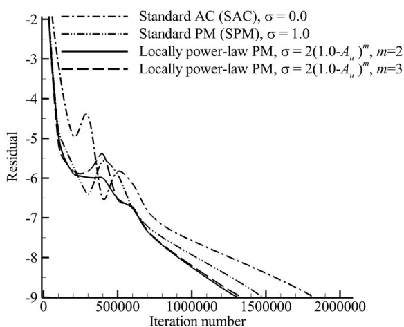
Fig. 20 Effect of the locally power-law PM on convergence rate around the NACA0012 hydrofoil at Re = 500 , \alpha = 15^\circ
