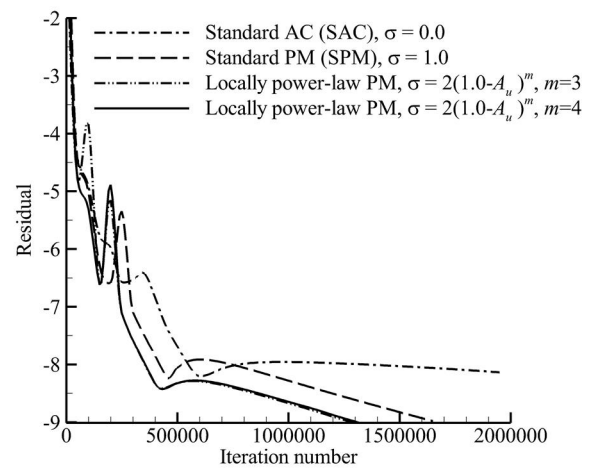
Fig. 22 Effect of the locally power-law PM on convergence rate around the NACA0012 hydrofoil at Re = 800 , \alpha = 15^\circ
