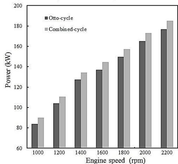
Fig. 18 The comparison between power of SI engine and suggested combined cycle
