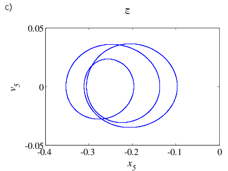
Fig. 18 Disk response: a) time series b) power spectra c) phase plane d) poincaré map with weight effect at \Omega = 0.32
