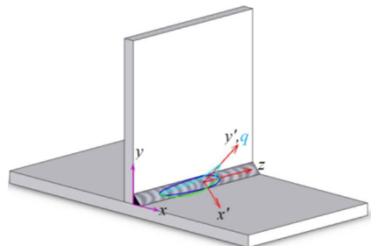
Fig. 7 Transformation of the coordinate system
