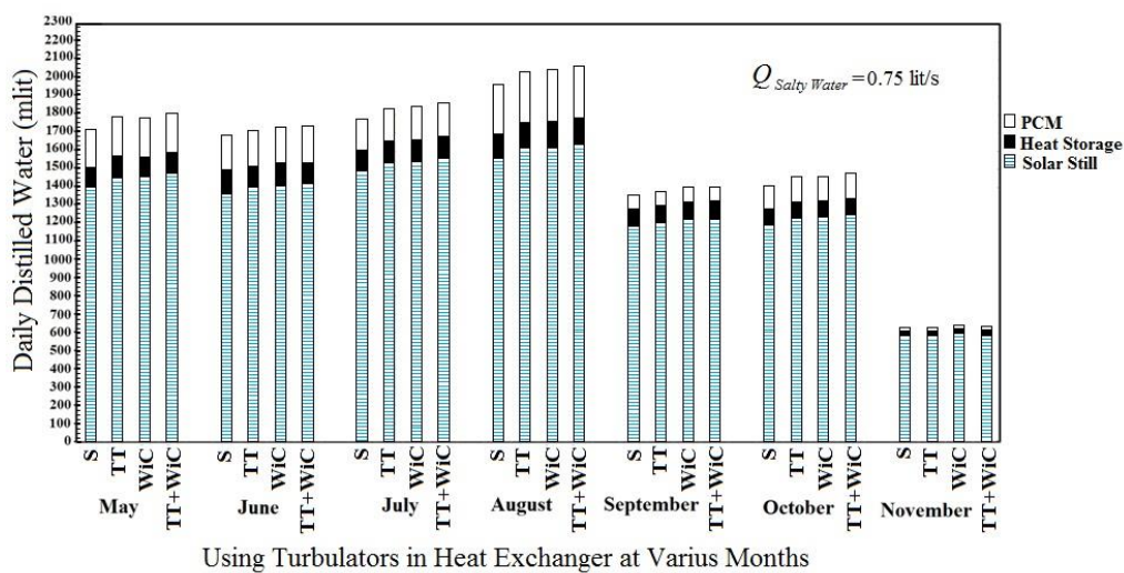
Fig. 17 Daily distilled water gain in using various turbulators and PCM at salty water flow rate 0.75lit/s
