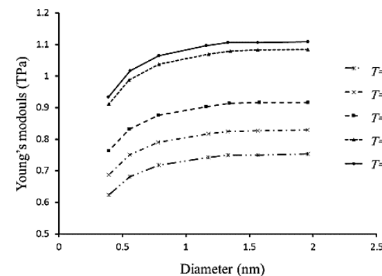
Fig. 6 Variations of Young's modulus in zigzag nanotubes with different diameters in different temperatures
