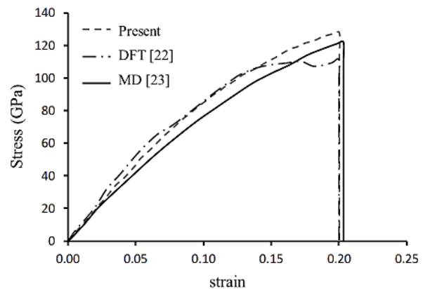
Fig. 5 Stress-Strain diagram in armchair nanotube (5,5) with current study in comparison to reference methods [22] & [23]
