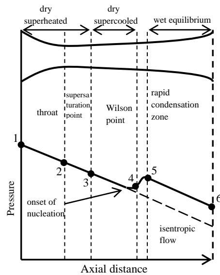
Fig. 1 Axial pressure distribution in a nozzle with spontaneous condensation
