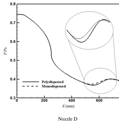
Fig. 6 Pressure distribution through Moore nozzles [10] centerline
