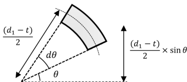
Fig. 3 Pipe element of integration
