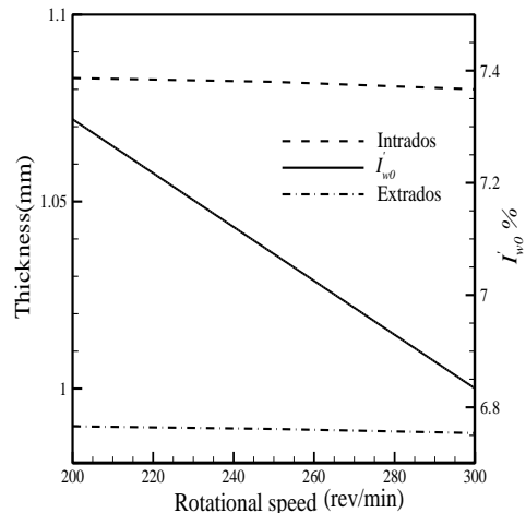
Fig. 14 Comparisons of tube thickness and I'_{w0} with different rotational speed
