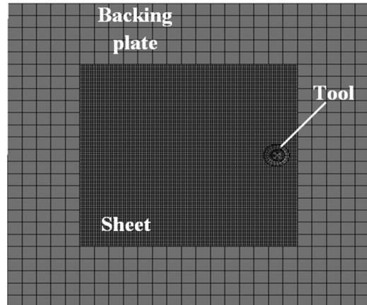
Fig.8 The finite element model of SPIF in Abaqus software
