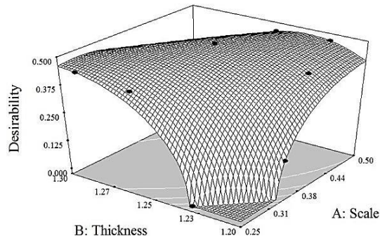
Fig. 12 Effects of design factors scale and thickness of tubes of both desirability for optimization problem cause of increases energy absorption
