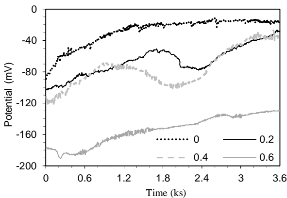
Fig. 12 Variations of open circuit potential values versus time for milled samples using tools with different flank wear.
