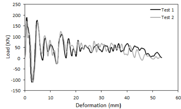
Fig. 12 Load-Deformation diagram for impact tests
