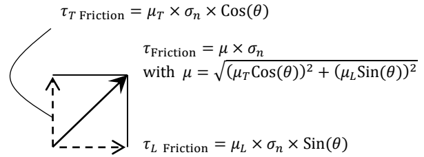
Fig. 7 Transverse shear caused by friction on fracture plane and its components in shear stress directions [19]
