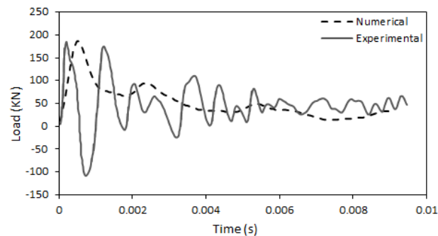
Fig. 13 comparison of numerical and experimental Load-Time diagrams
