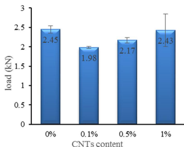
Fig.11 Maximum contact force at different percentages of nanotube
