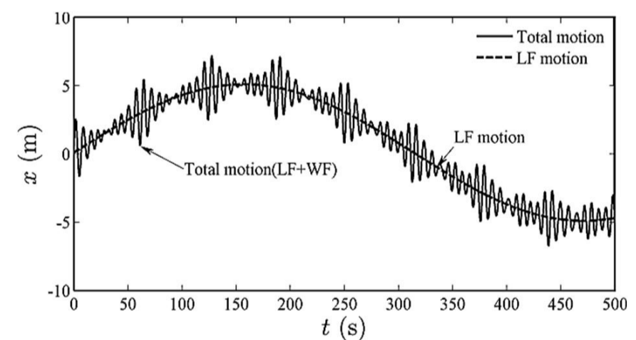
Fig. 3 Example of a marine vessel motion. The total motion can be thought of as the superposition of a low-frequency (LF) and a zero-mean oscillatory wave-frequency (WF) component
