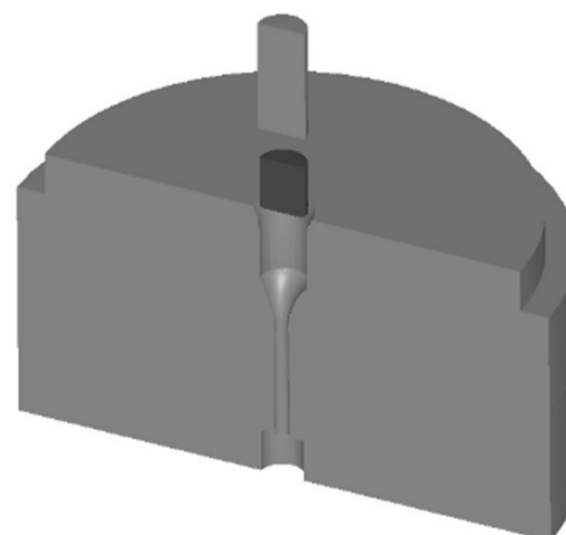
Fig. 3 Model of billet, punch and die
