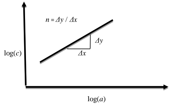
Fig. 12 How to calculate factor n in a compliance calibration method [14]
