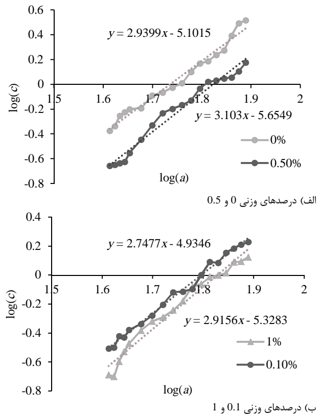
Fig. 13 Comparison the value of n in log(c)-log(a) diagram a) 0 wt % and 0.5 wt % b) 0.1 wt % and 1 wt %
