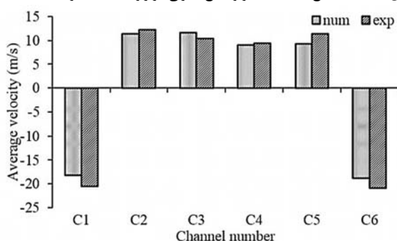
Fig. 7 Comparison of current study and experiment results in 90° wind incident angle
