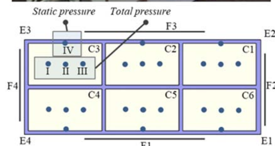
Fig. 5 location of pitot and statics in all windcatcher channels
