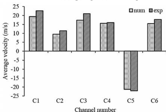
Fig. 8 Comparison of current study and experiment results in 180° wind incident angle
