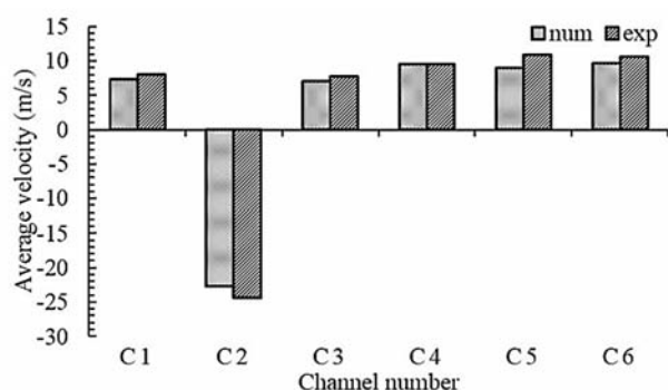
Fig. 6 Comparison of current study and experiment results in zero wind incident angle
