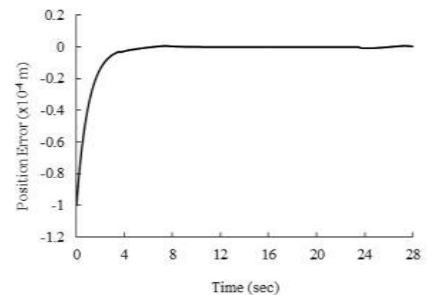
Fig. 13 Position error of the system in interaction with the soft tissue
