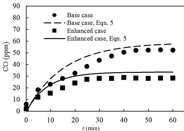
Fig. 2 Comparison of numerical results and Eqn. (5) [10]
