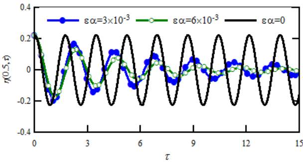
Fig. 3. The effect of the viscoelastic parameters on dynamic response of the simply supported fluid conveying pipe for u = 3
