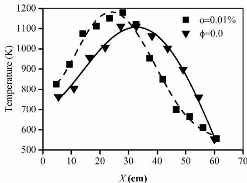
Fig. 6 The effect of nanoparticles mass fraction (0.01%) on the flame distribution along the flame axis
