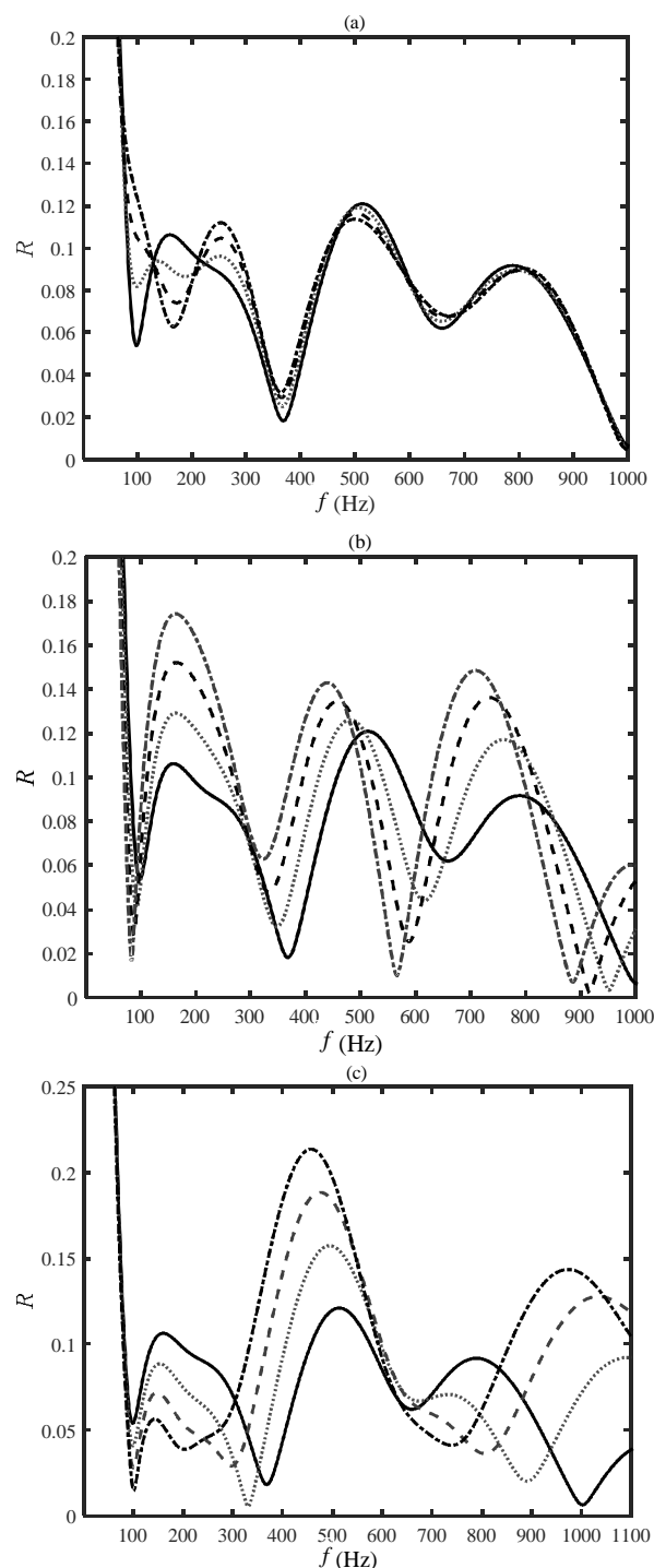
Fig. 7 The effect of air gap on sound pressure reflection coefficient for optimum structure 1 in Table 3, (a) if the air gap has been located between the wall and third layer, (b) if the air gap has been located between the third and second layers, (c) if the air gap has been located between the second and first layers. ( — without air gap, ..... 3 cm air gap, - - - 6 cm air gap, - . - 9 cm air gap)
