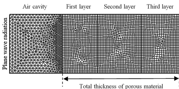
Fig. 2 Final mesh of the structure
