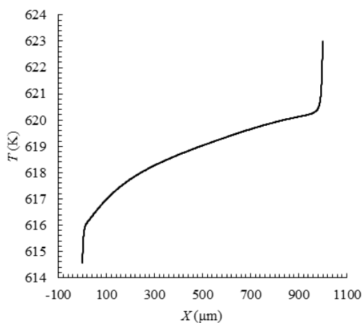
Fig. 7 Temperature distribution along the microchannel for D=10 \mu m and A=40 \mu m
