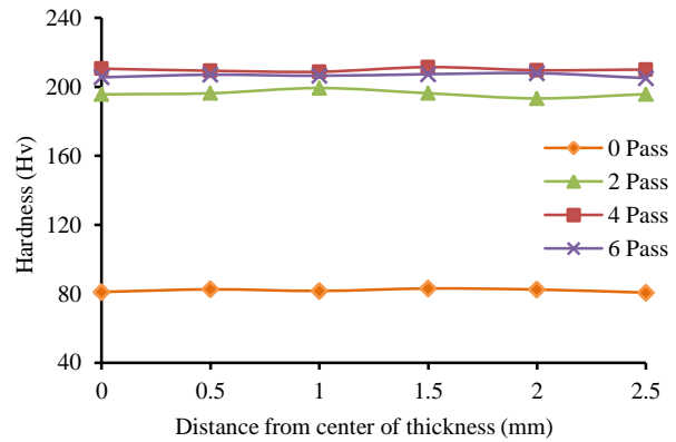
Fig. 7 Vickers hardness number plot for ECAP performed samples with specific number of pass
