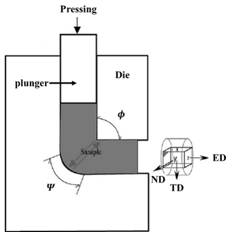
Fig. 1 Schematic illustration of the ECAP facility showing the angles \phi and \psi [9]
