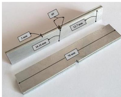
Fig. 2 Charpy impact test specimens made from FML
