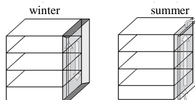
Fig. 1 The performance of double skin façade in winter and summer
