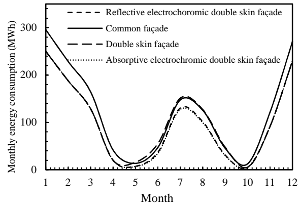
Fig. 4 The comparison of monthly energy consumption for four different facade
