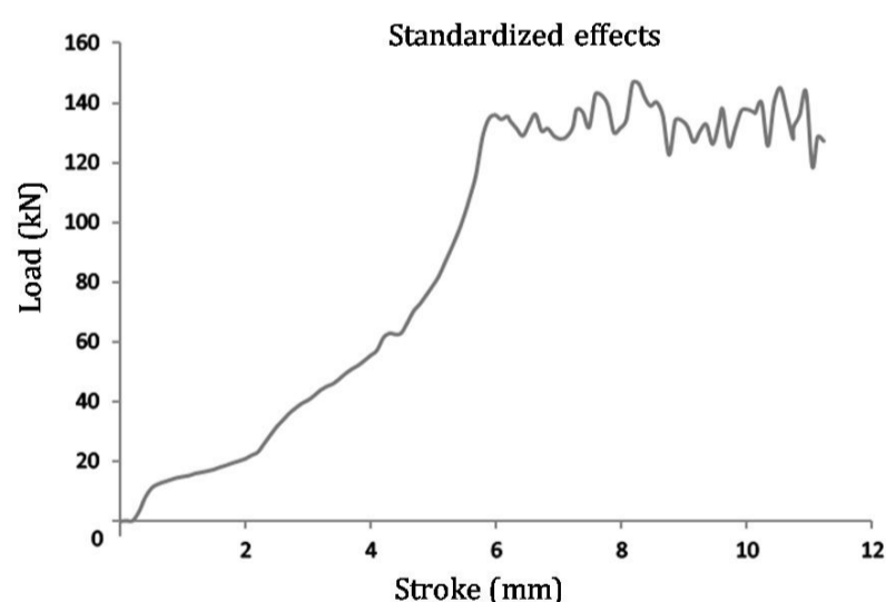
Fig. 8 The force required for blade preforms extrusion
