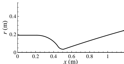
Fig. 1 (a) STAR-27 Nozzle and Engine photograph, (b) STAR-27 Nozzle Profile [14]
