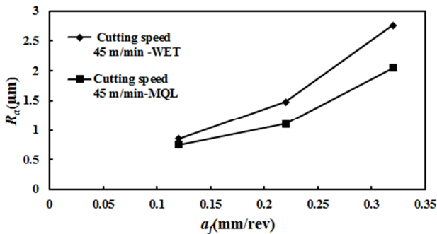
Fig. 13 Comparison surface roughness of two methods MQL and wet in cutting speed of 45 meters per minute and variable feed rate
