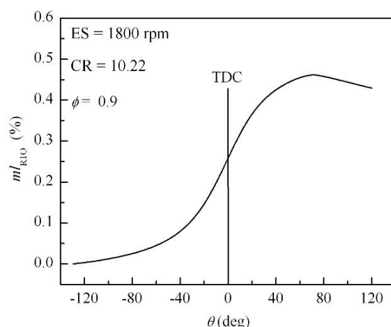
Fig. 9 Percentage of mass lost from the first ring orifice versus crank angle estimated from polytopic model
