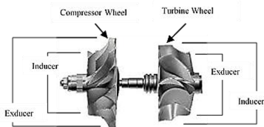
Fig. 5 Geometric characteristics in defining Trim parameter
