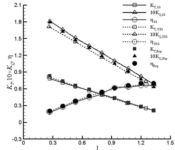
Fig. 7 Comparison of the steady and unsteady results with the experimental data
