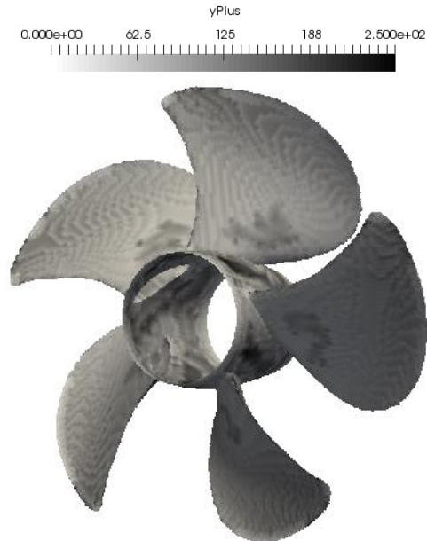
Fig. 6 The y^+ contour on the propeller at the fine grid at J = 1.06
