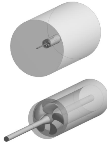
Fig. 2 General overview of the solution domain (top) and near & wake region of the propeller (bottom)
