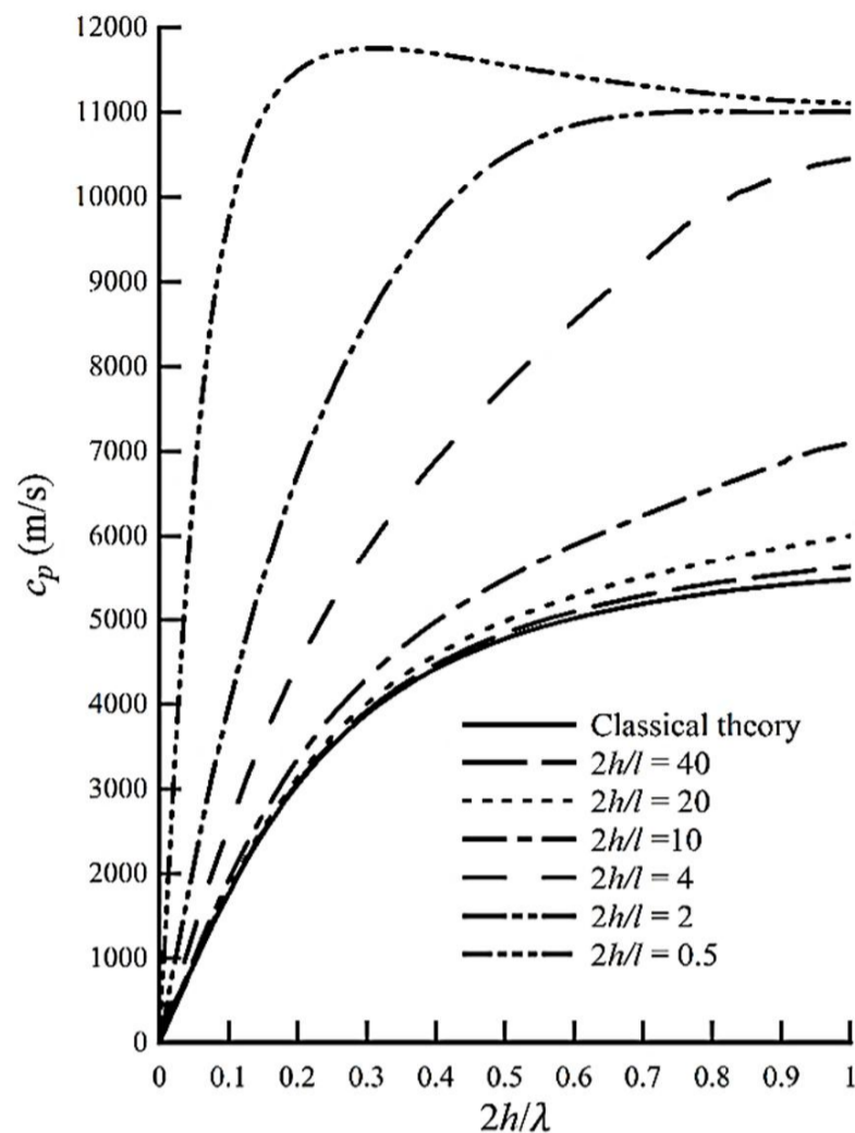
Fig. 3 Dispersion curve of phase velocity for first anti-symmetric mode in different thickness to characteristic length ratios
