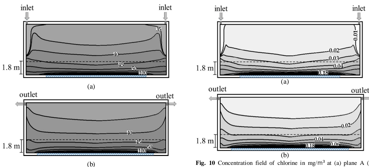
Fig. 11 Relative humidity field (%) (a) plane A (b) plane B
