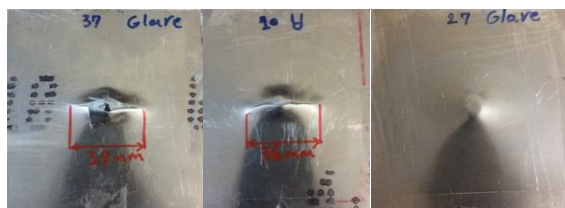
Fig. 14 Bottom layer of aluminum tear on specimen No. 27 (flat projectile), No. 10 (hemispherical projectile) and No. 37 (conical 90° projectile) in 40J impact.
