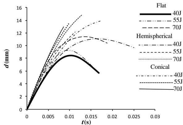
Fig. 8 Deflection-time curve in flat, hemispherical and conical 90° projectile
